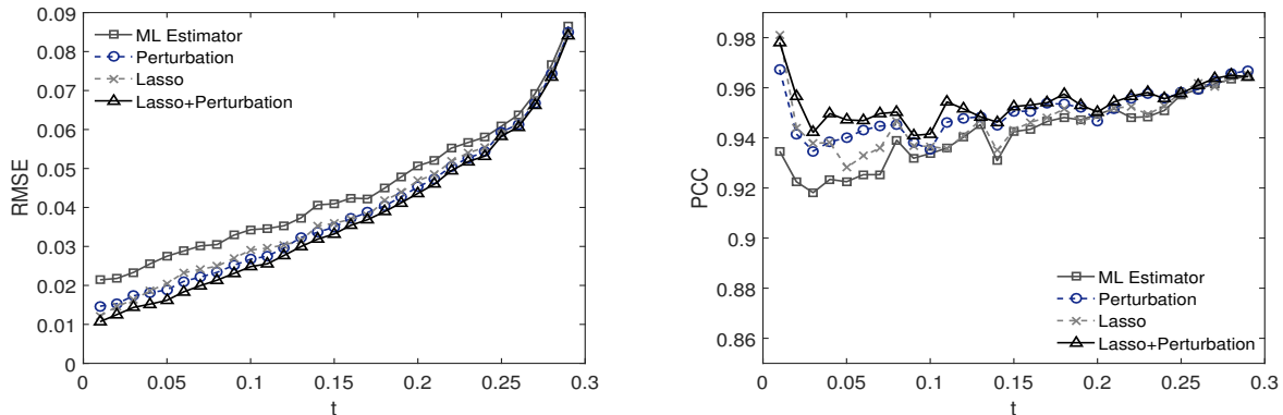
Figure 10 RMSE (left panel) and PCC (right panel) of the ML, lasso, perturbation and lasso+perturbation estimators in Example 3
