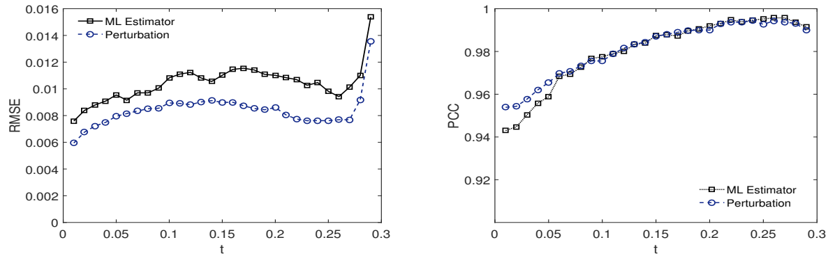
Figure 5 RMSE (left panel) and PCC (right panel) of the ML and perturbation estimators in Example 1
