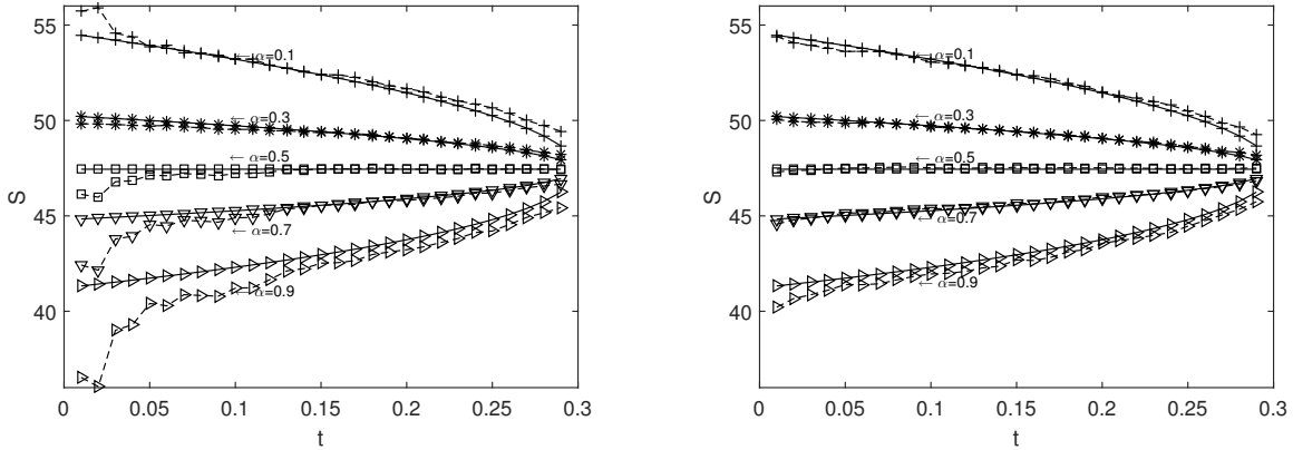
Figure 3 The boundaries for different \alpha values using the original (left) and perturbed (right) sample paths. The solid lines are the true boundaries, and the dashed lines are the estimated boundaries via logistic regression
