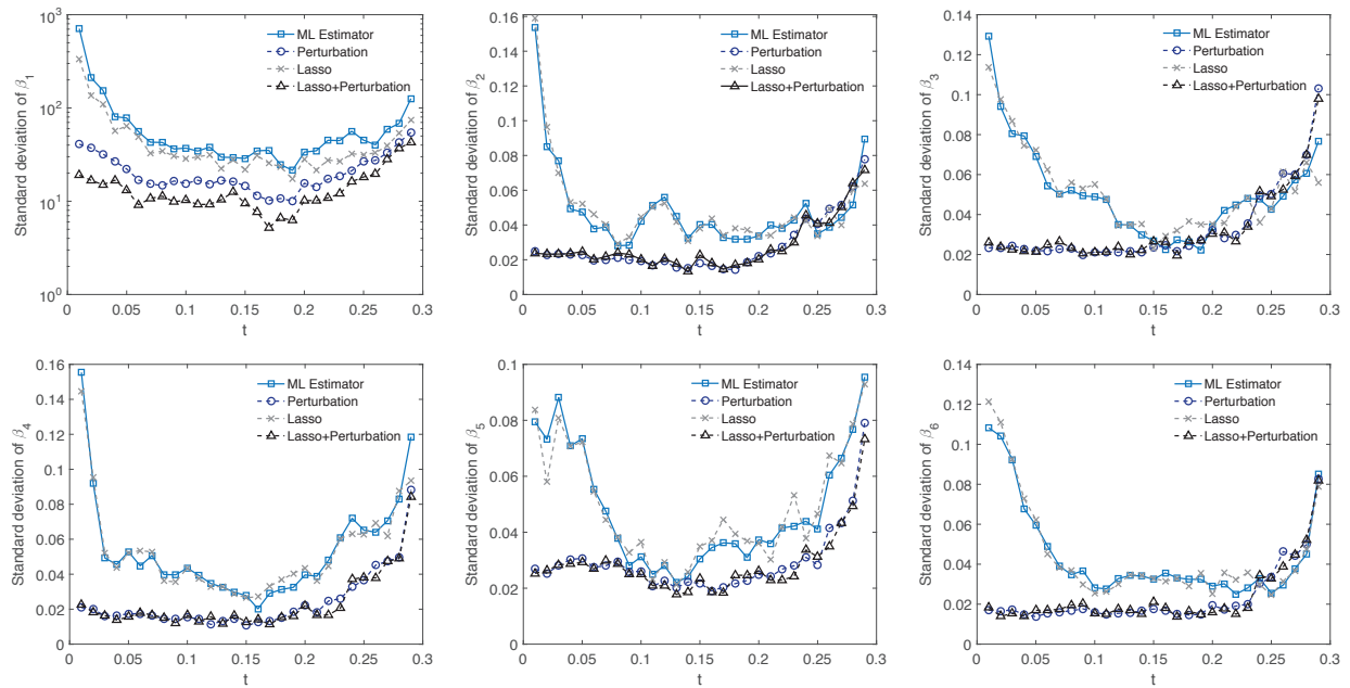
Figure 7 Standard deviations of the ML, lasso, perturbation and lasso+perturbation estimators of \beta_1, \dots, \beta_6 in Example 2
