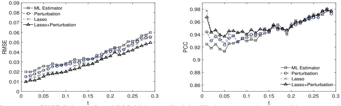
Figure 11 RMSE (left panel) and PCC (right panel) of the ML, lasso, perturbation and lasso+perturbation estimators in Example 3 with square terms
