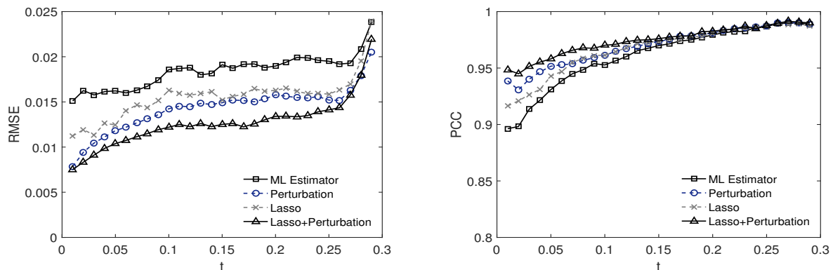
Figure 9 RMSE (left panel) and PCC (right panel) of the ML, lasso, perturbation and lasso+perturbation estimators in Example 2
