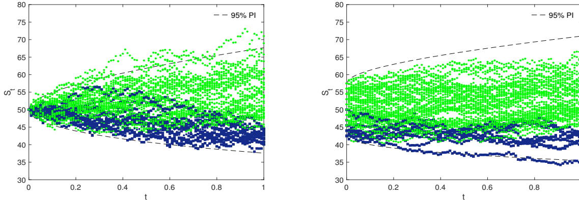
Figure 2 The default paths (darker color) and the non-default paths (lighter color) before and after perturbing the initial value
