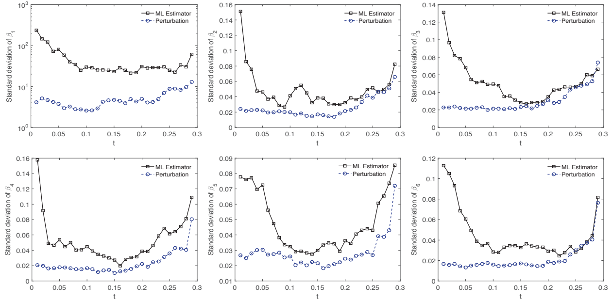
Figure 4 Standard deviations of the ML and perturbation estimators in Example 1
